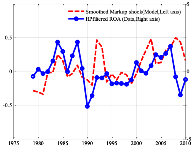
FIG. 4. Smoothed Markup Shock and HP-filtered ROA
